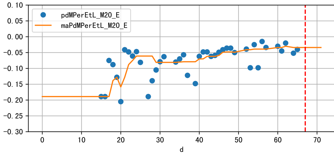
Daily %DeltaM and %DeltaM/1000ml ETcIdef for M20_E (-1.6%/D, -3.4%/1000ml ET)
