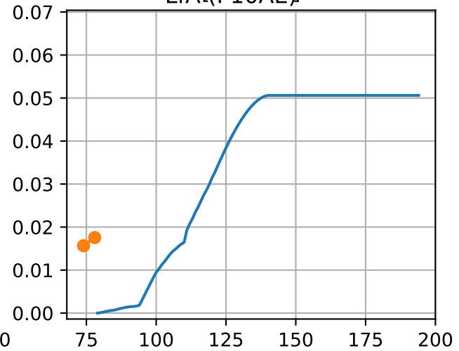
LfA(['S1L16'])
