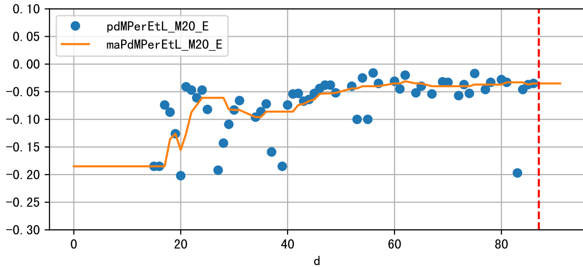
Daily %DeltaM and %DeltaM/1000ml ETcIdef for M20_E (-1.9%/D, -3.5%/1000ml ET)
