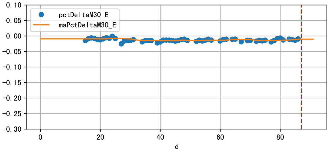
Daily %DeltaM and %DeltaM/1000ml ETcIdef for M30_E (-1.0%/D, -2.4%/1000ml ET)
