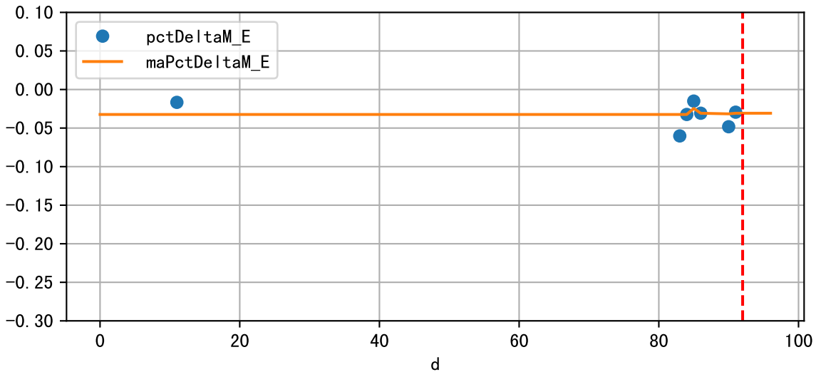
Daily %DeltaM and %DeltaM/1000ml ETcIdef for M_E (-3.1%/D, -12.1%/1000ml ET)
