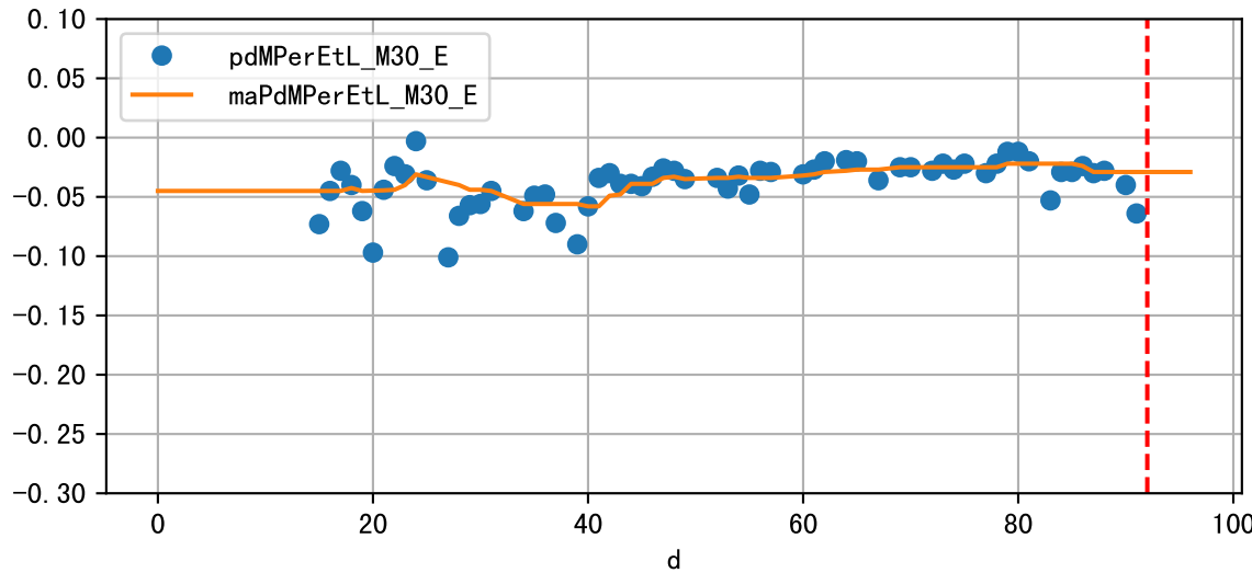
Daily %DeltaM and %DeltaM/1000ml ETcIdef for M30_E (-1.2%/D, -2.9%/1000ml ET)
