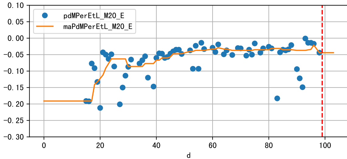
Daily %DeltaM and %DeltaM/1000ml ETcIdef for M20_E (-2.7%/D, -4.4%/1000ml ET)
