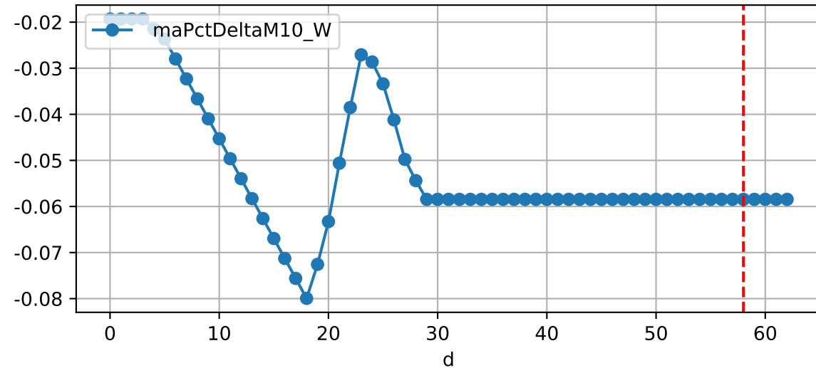
Daily %DeltaM and %DeltaM/1000ml ETcldef for M10_W (-5.8%/D, -3.9%/1000ml ET)
