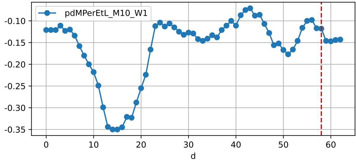
Daily %DeltaM and %DeltaM/1000ml ETcldef for M10_W1 (-17.8%/D, -11.8%/1000ml ET)
