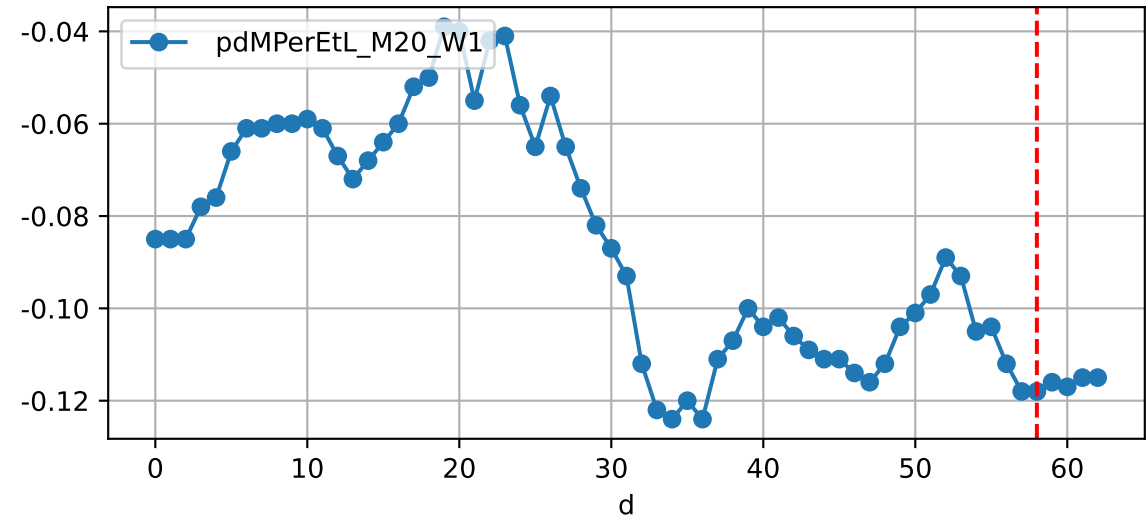
Daily %DeltaM and %DeltaM/1000ml ETcldef for M20_W1 (-17.9%/D, -11.8%/1000ml ET)
