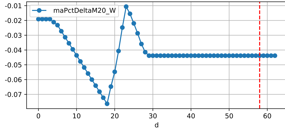
Daily %DeltaM and %DeltaM/1000ml ETcldef for M20_W (-4.4%/D, -2.9%/1000ml ET)
