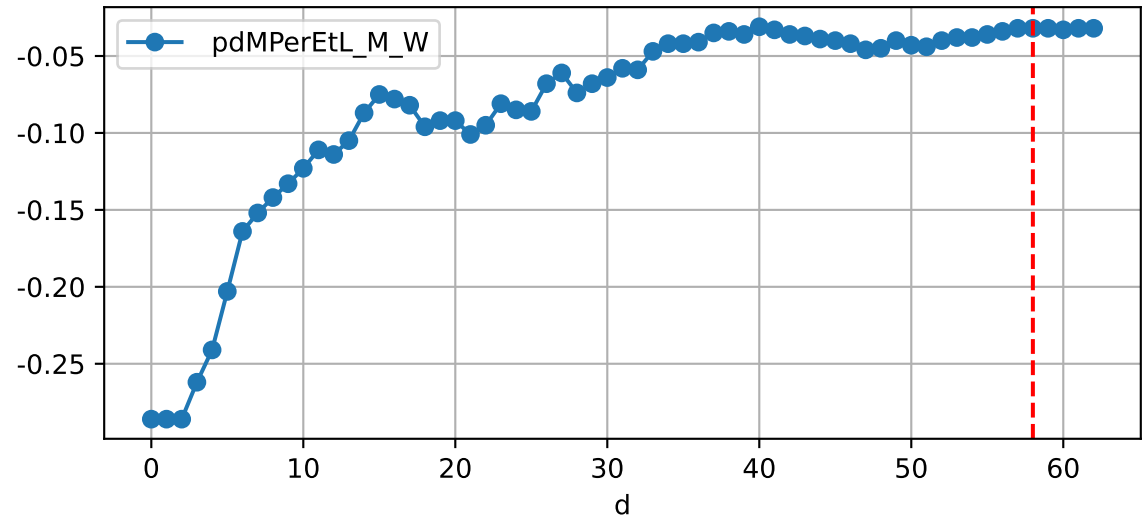
Daily %DeltaM and %DeltaM/1000ml ETcIdef for M_W (-4.9%/D, -3.2%/1000ml ET)
