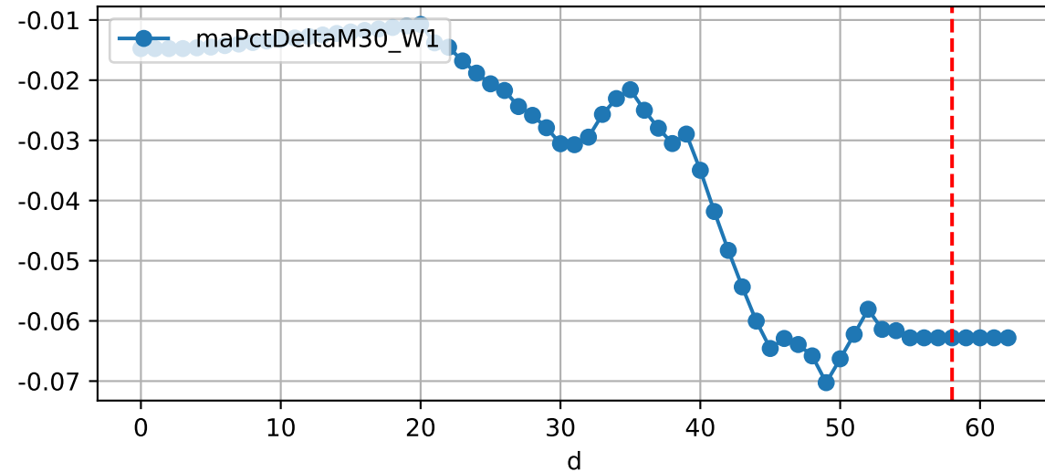
Daily %DeltaM and %DeltaM/1000ml ETcldef for M30_W1 (-6.3%/D, -4.2%/1000ml ET)
