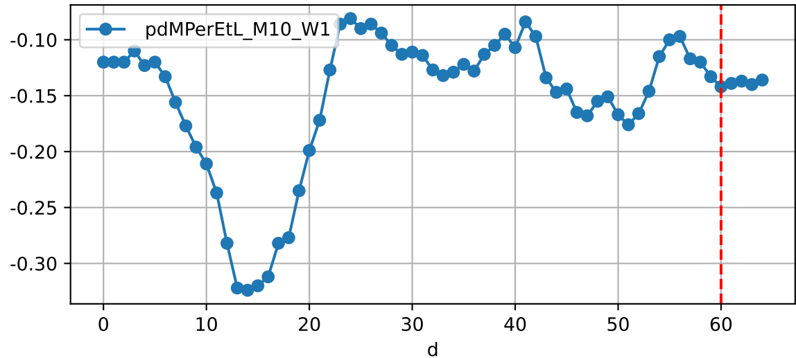
Daily %DeltaM and %DeltaM/1000ml ETcldef for M10_W1 (-22.5%/D, -14.2%/1000ml ET)
