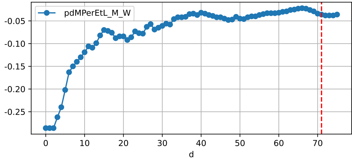
Daily %DeltaM and %DeltaM/1000ml ETcIdef for M_W (-5.9%/D, -3.6%/1000ml ET)
