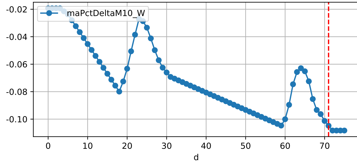
Daily %DeltaM and %DeltaM/1000ml ETcldef for M10_W (-10.5%/D, -6.4%/1000ml ET)
