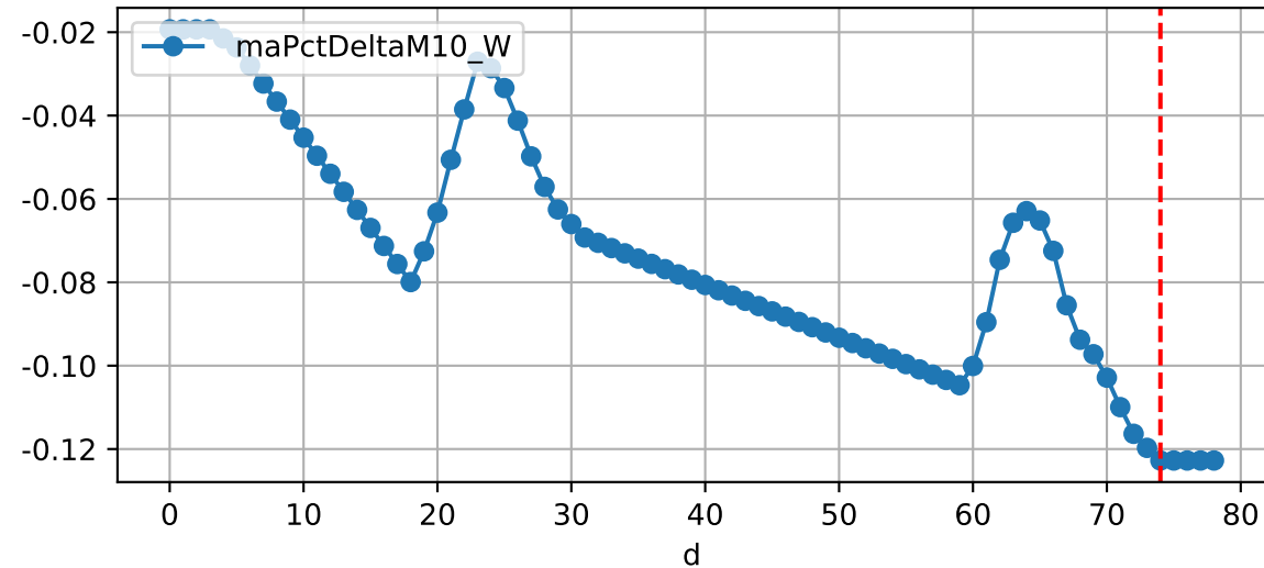
Daily %DeltaM and %DeltaM/1000ml ETcldef for M10_W (-12.3%/D, -8.2%/1000ml ET)
