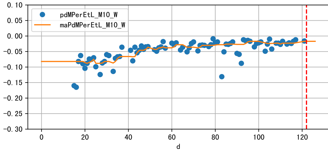
Daily %DeltaM and %DeltaM/1000ml ETcIdef for M10_W (-1.6%/D, -1.7%/1000ml ET)
