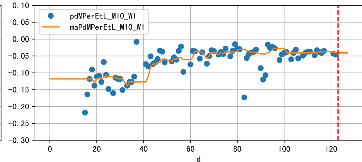
Daily %DeltaM and %DeltaM/1000ml ETcIdef for M10_W1 (-3.1%/D, -4.1%/1000ml ET)
