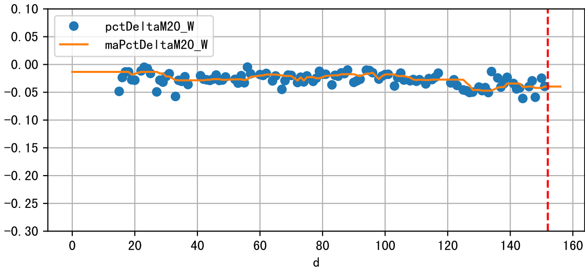
Daily %DeltaM and %DeltaM/1000ml ETcIdef for M20_W (-4.0%/D, -3.7%/1000ml ET)
