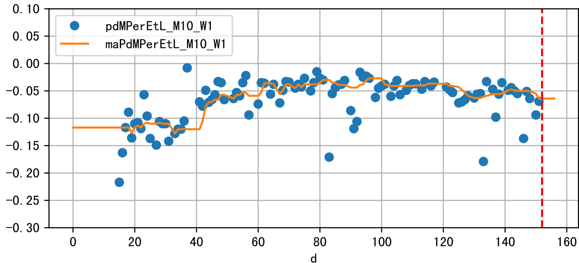
Daily %DeltaM and %DeltaM/1000ml ETcldef for M10_W1 (-6.3%/D, -6.4%/1000ml ET)
