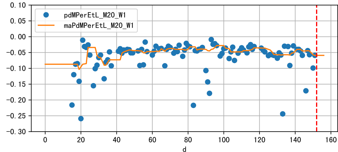
Daily %DeltaM and %DeltaM/1000ml ETcIdef for M20_W1 (-6.2%/D, -5.9%/1000ml ET)
