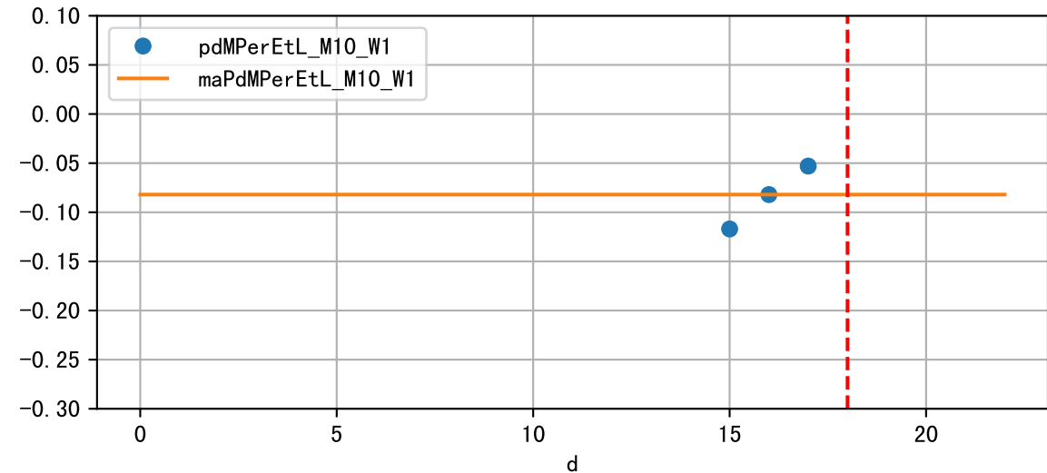
Daily %DeltaM and %DeltaM/1000ml ETcIdef for M10_W1 (-3.1%/D, -8.2%/1000ml ET)
