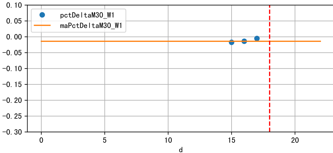
Daily %DeltaM and %DeltaM/1000ml ETcIdef for M30_W1 (-1.4%/D, -3.8%/1000ml ET)
