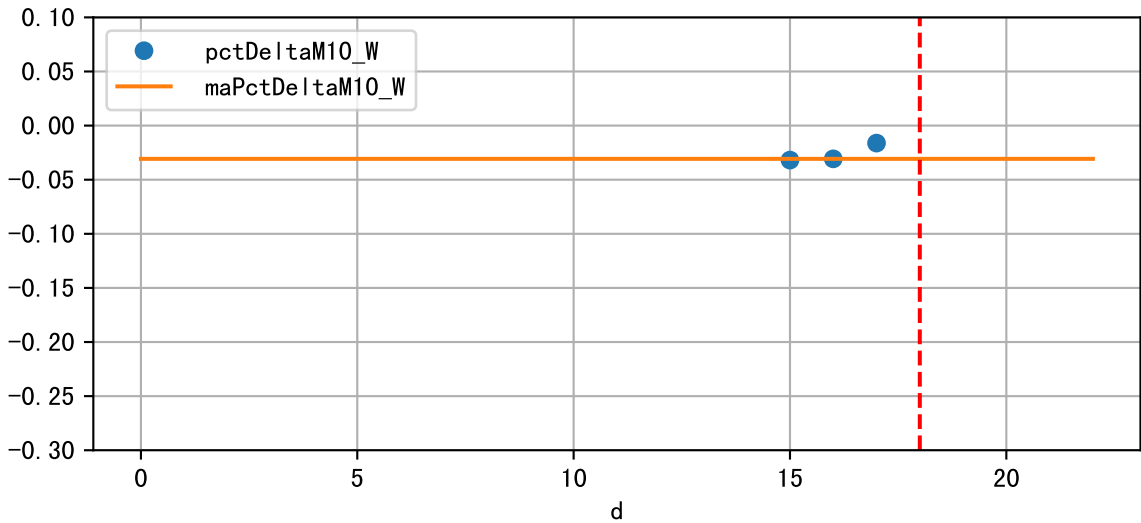
Daily %DeltaM and %DeltaM/1000ml ETcIdef for M10_W (-3.1%/D, -8.3%/1000ml ET)
