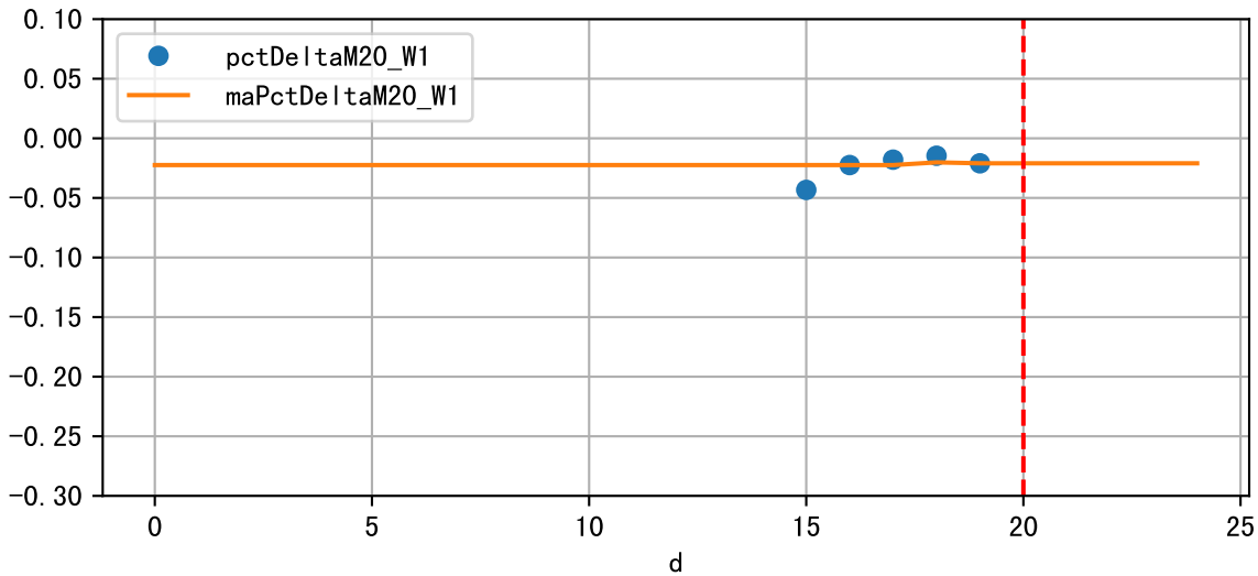
Daily %DeltaM and %DeltaM/1000ml ETcIdef for M20_W1 (-2.1%/D, -5.6%/1000ml ET)
