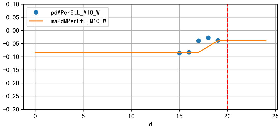
Daily %DeltaM and %DeltaM/1000ml ETcIdef for M10_W (-1.7%/D, -3.9%/1000ml ET)
