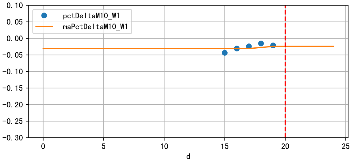
Daily %DeltaM and %DeltaM/1000ml ETcIdef for M10_W1 (-2.4%/D, -5.6%/1000ml ET)
