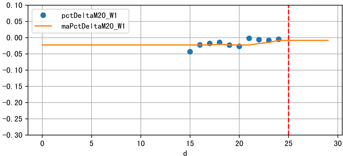
Daily %DeltaM and %DeltaM/1000ml ETcldef for M20_W1 (-0.8%/D, -2.1%/1000ml ET)
