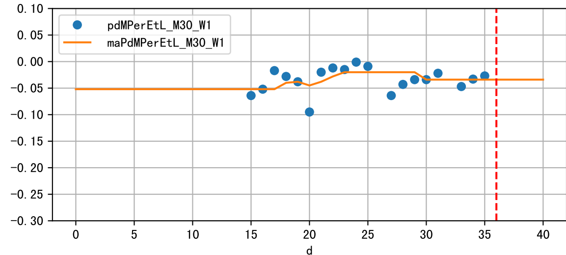
Daily %DeltaM and %DeltaM/1000ml ETcIdef for M30_W1 (-1.4%/D, -3.4%/1000ml ET)
