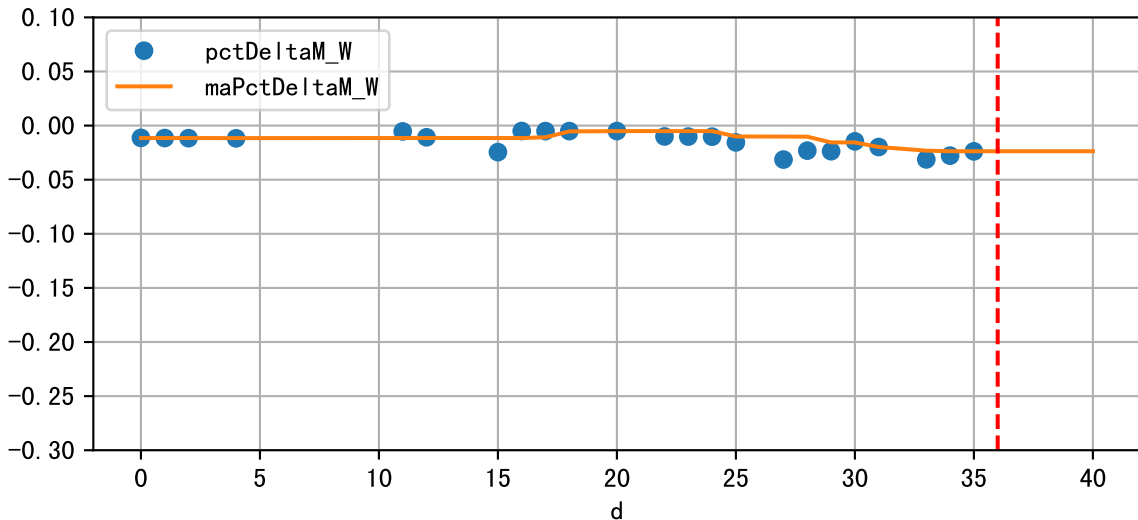
Daily %DeltaM and %DeltaM/1000ml ETcIdef for M_W (-2.4%/D, -5.4%/1000ml ET)
