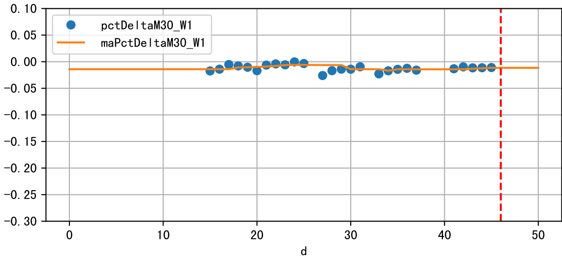
Daily %DeltaM and %DeltaM/1000ml ETcIdef for M30_W1 (-1.2%/D, -4.9%/1000ml ET)
