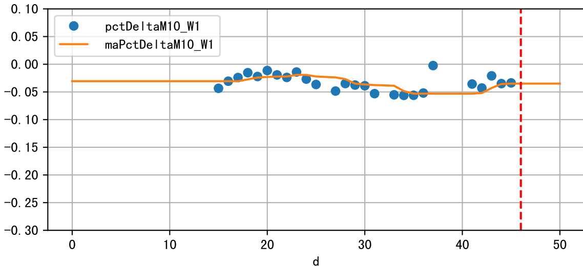
Daily %DeltaM and %DeltaM/1000ml ETcIdef for M10_W1 (-3.5%/D, -13.2%/1000ml ET)
