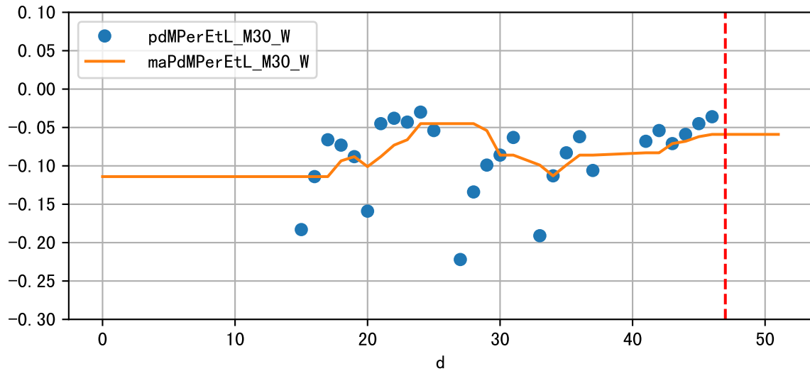
Daily %DeltaM and %DeltaM/1000ml ETcIdef for M30_W (-1.6%/D, -5.9%/1000ml ET)
