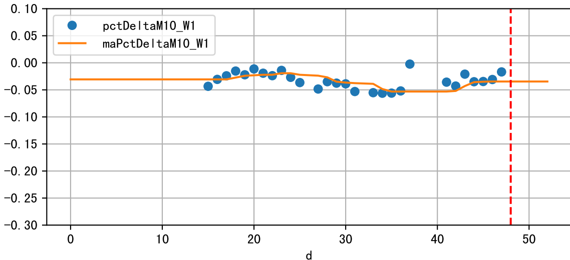
Daily %DeltaM and %DeltaM/1000ml ETcIdef for M10_W1 (-3.5%/D, -11.4%/1000ml ET)
