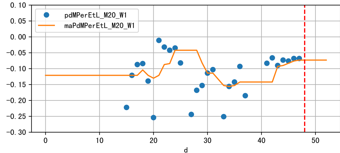
Daily %DeltaM and %DeltaM/1000ml ETcldef for M20_W1 (-2.2%/D, -7.3%/1000ml ET)
