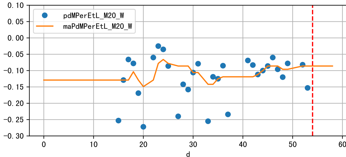
Daily %DeltaM and %DeltaM/1000ml ETcIdef for M20_W (-2.7%/D, -8.6%/1000ml ET)
