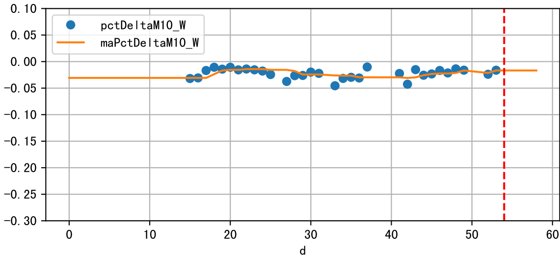
Daily %DeltaM and %DeltaM/1000ml ETcIdef for M10_W (-1.7%/D, -7.2%/1000ml ET)
