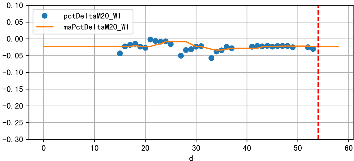
Daily %DeltaM and %DeltaM/1000ml ETcIdef for M20_W1 (-2.3%/D, -7.6%/1000ml ET)
