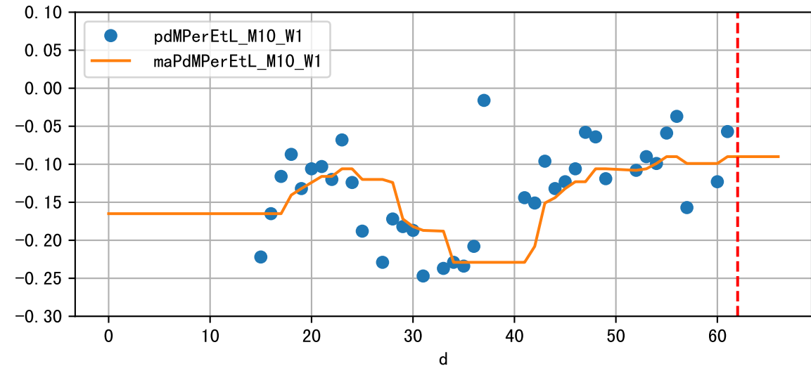
Daily %DeltaM and %DeltaM/1000ml ETcIdef for M10_W1 (-1.9%/D, -9.0%/1000ml ET)
