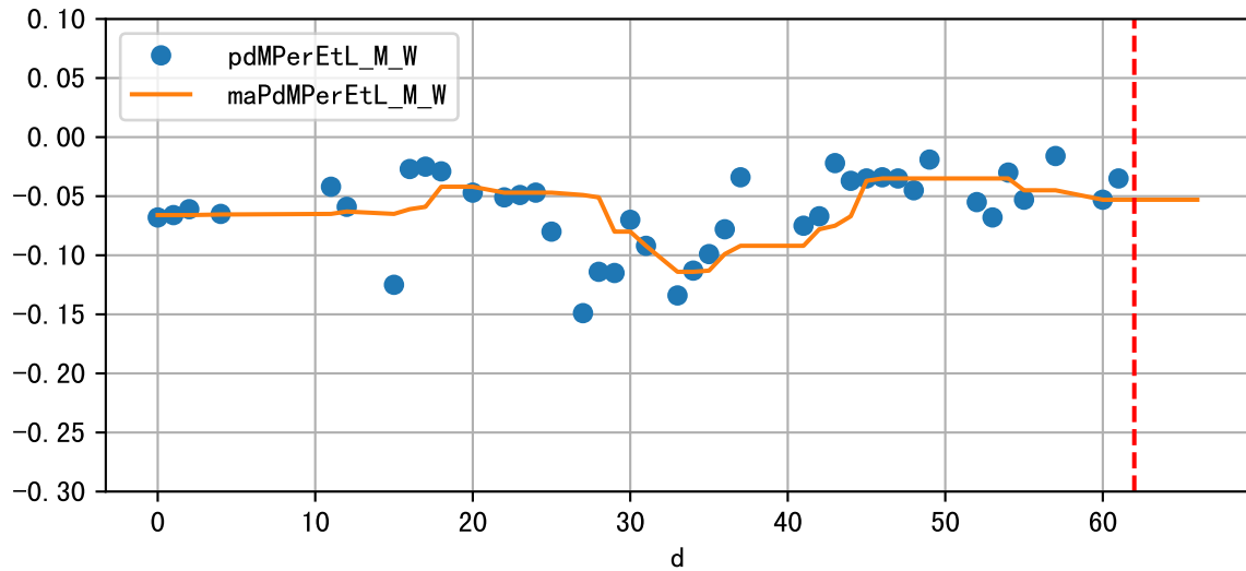
Daily %DeltaM and %DeltaM/1000ml ETcIdef for M_W (-1.0%/D, -5.3%/1000ml ET)
