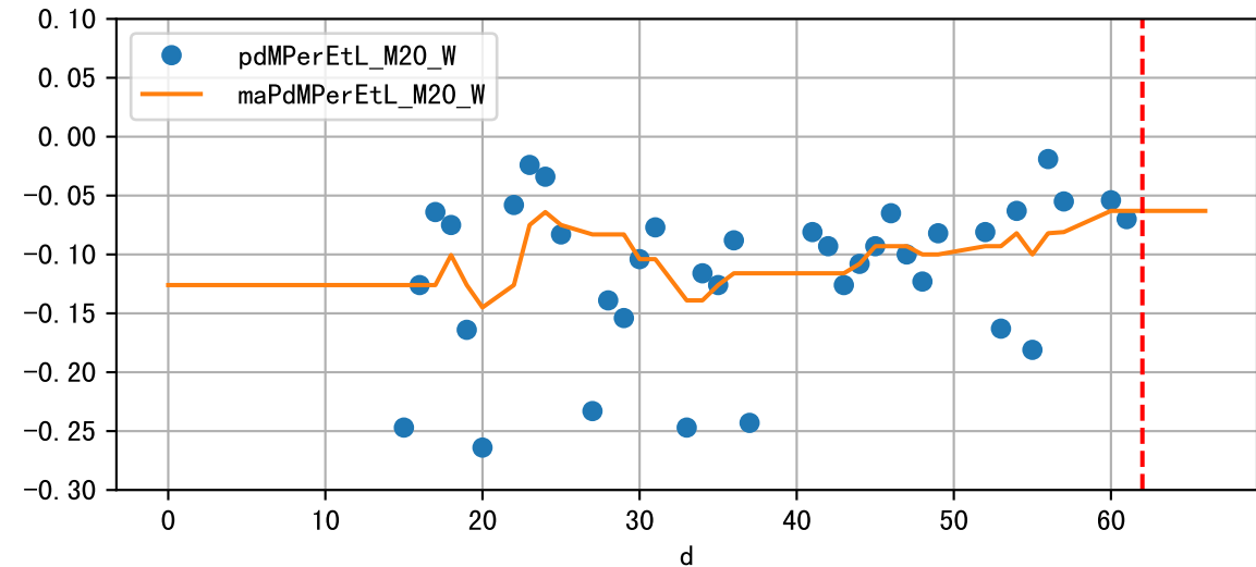
Daily %DeltaM and %DeltaM/1000ml ETcIdef for M20_W (-1.8%/D, -6.3%/1000ml ET)
