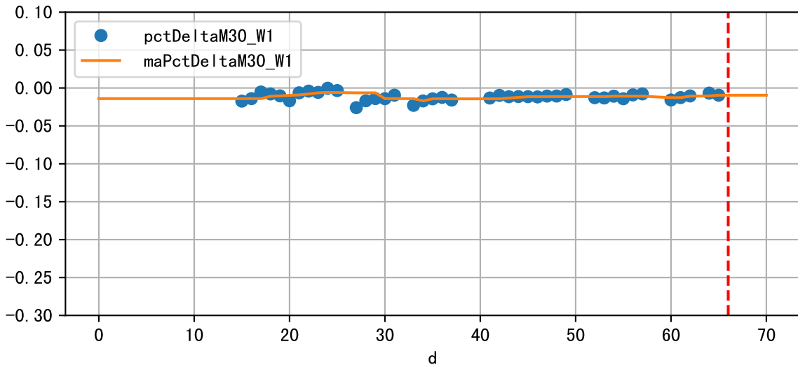
Daily %DeltaM and %DeltaM/1000ml ETcIdef for M30_W1 (-1.0%/D, -4.7%/1000ml ET)
