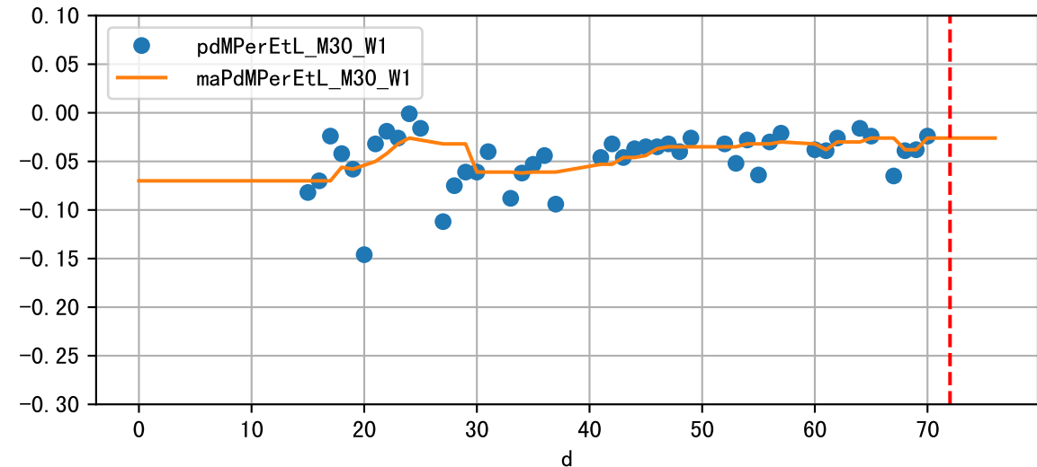
Daily %DeltaM and %DeltaM/1000ml ETcIdef for M30_W1 (-1.1%/D, -2.6%/1000ml ET)
