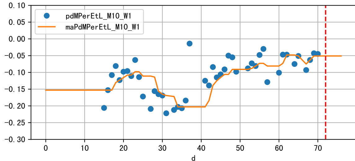
Daily %DeltaM and %DeltaM/1000ml ETcIdef for M10_W1 (-2.1%/D, -5.1%/1000ml ET)
