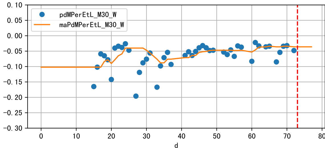
Daily %DeltaM and %DeltaM/1000ml ETcIdef for M30_W (-1.6%/D, -3.6%/1000ml ET)
