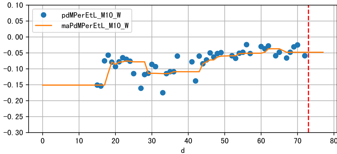
Daily %DeltaM and %DeltaM/1000ml ETcIdef for M10_W (-2.3%/D, -4.8%/1000ml ET)
