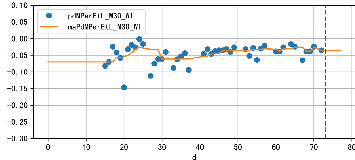
Daily %DeltaM and %DeltaM/1000ml ETcIdef for M30_W1 (-1.7%/D, -3.5%/1000ml ET)
