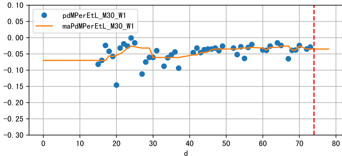
Daily %DeltaM and %DeltaM/1000ml ETcldef for M30_W1 (-1.7%/D, -3.5%/1000ml ET)
