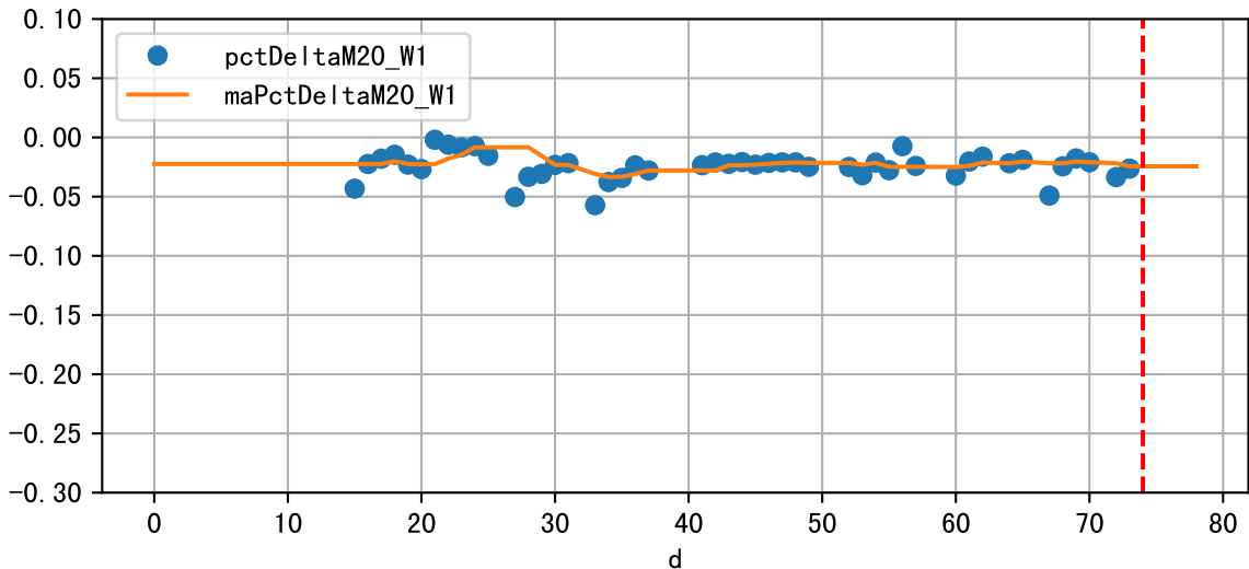
Daily %DeltaM and %DeltaM/1000ml ETcIdef for M20_W1 (-2.4%/D, -5.1%/1000ml ET)
