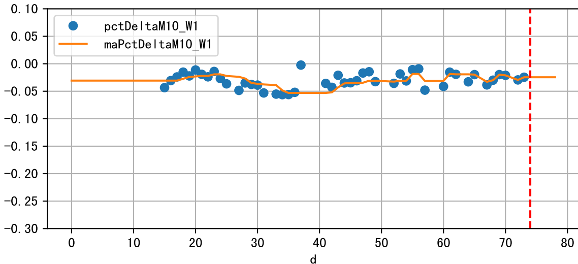
Daily %DeltaM and %DeltaM/1000ml ETcIdef for M10_W1 (-2.5%/D, -5.1%/1000ml ET)
