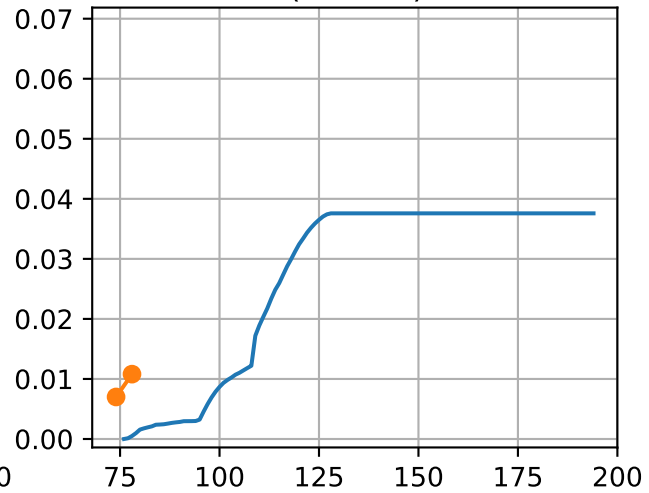
LfA (['S1L15'])
