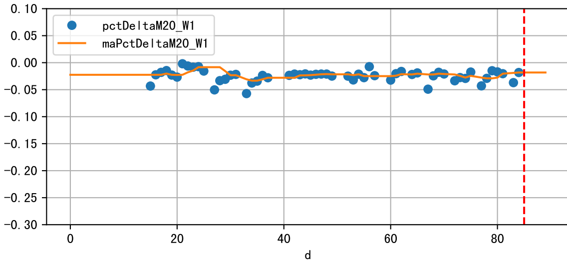
Daily %DeltaM and %DeltaM/1000ml ETcIdef for M20_W1 (-1.8%/D, -3.8%/1000ml ET)
