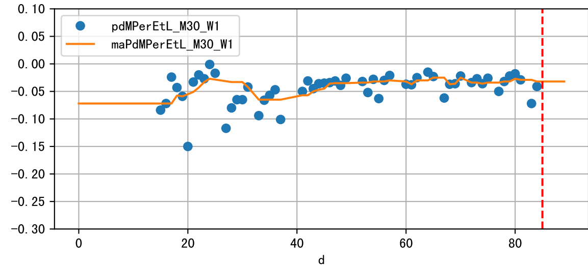
Daily %DeltaM and %DeltaM/1000ml ETcIdef for M30_W1 (-1.6%/D, -3.2%/1000ml ET)
