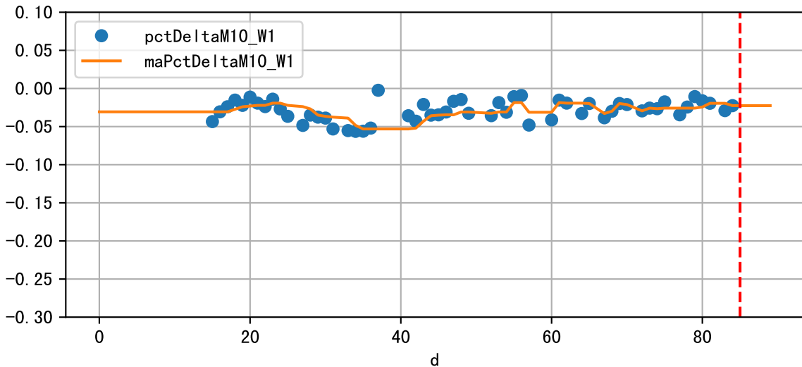
Daily %DeltaM and %DeltaM/1000ml ETcIdef for M10_W1 (-2.3%/D, -4.3%/1000ml ET)
