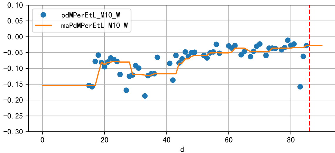
Daily %DeltaM and %DeltaM/1000ml ETcIdef for M10_W (-1.3%/D, -2.8%/1000ml ET)
