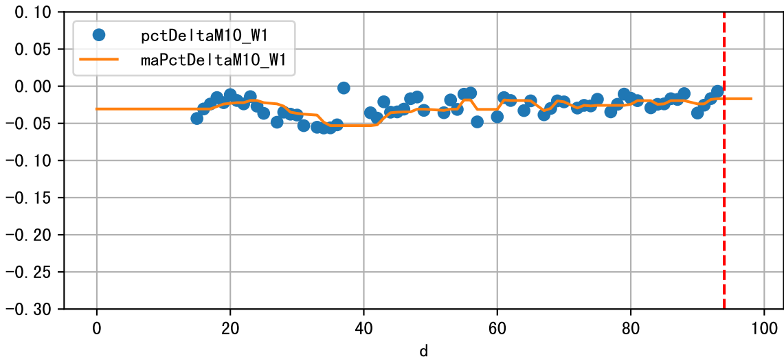
Daily %DeltaM and %DeltaM/1000ml ETcIdef for M10_W1 (-1.7%/D, -4.6%/1000ml ET)
