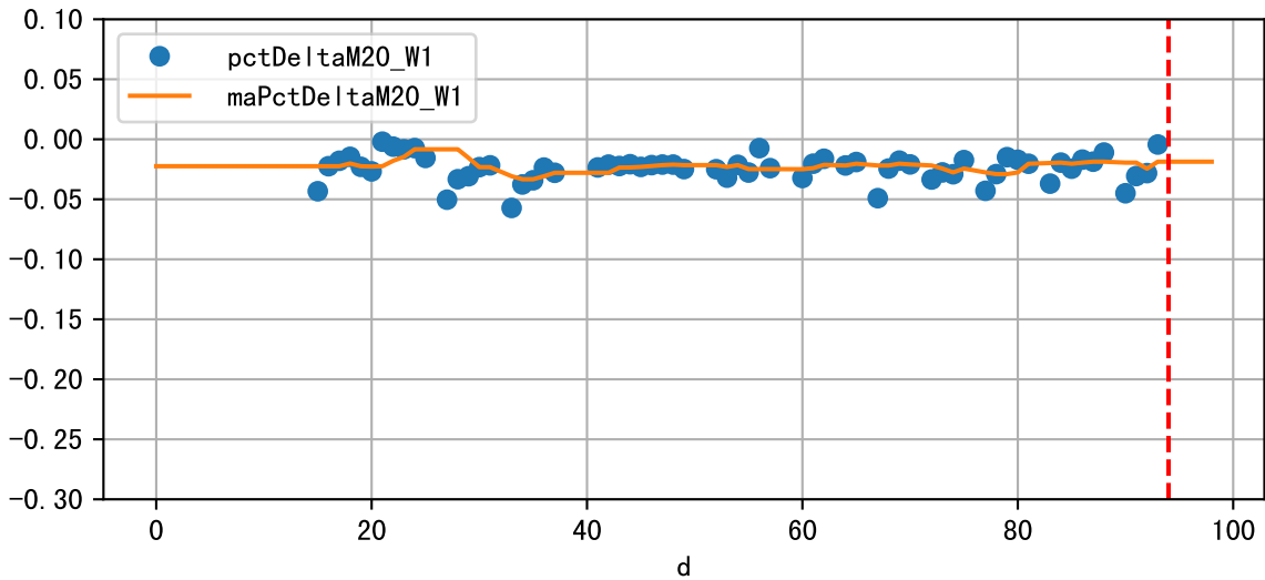
Daily %DeltaM and %DeltaM/1000ml ETcIdef for M20_W1 (-1.9%/D, -4.6%/1000ml ET)
