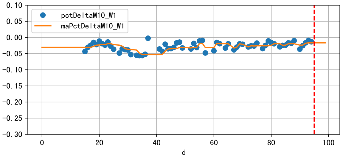
Daily %DeltaM and %DeltaM/1000ml ETcIdef for M10_W1 (-1.7%/D, -4.4%/1000ml ET)
