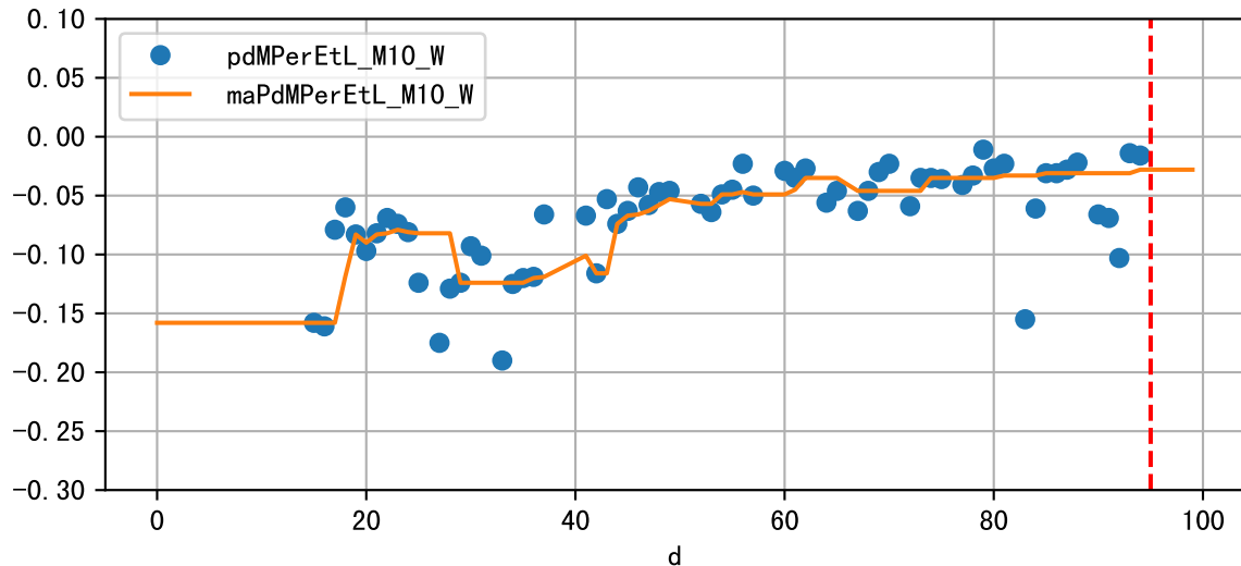
Daily %DeltaM and %DeltaM/1000ml ETcIdef for M10_W (-1.1%/D, -2.8%/1000ml ET)
