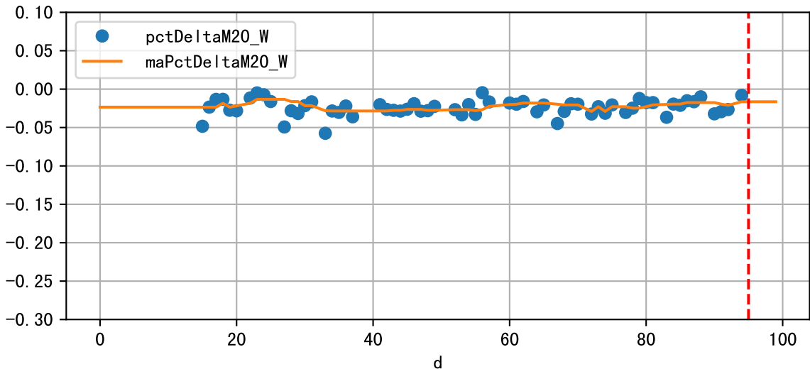
Daily %DeltaM and %DeltaM/1000ml ETcIdef for M20_W (-1.6%/D, -4.1%/1000ml ET)
