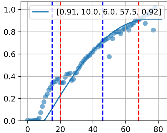
M_W d39 ([58.0, 2.6, -32.0] fdu=46.0)
