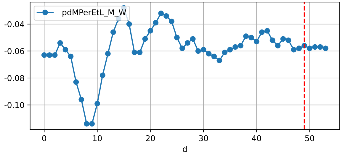
Daily %DeltaM and %DeltaM/1000ml ETcIdef for M_W (-7.7%/D, -5.6%/1000ml ET)
