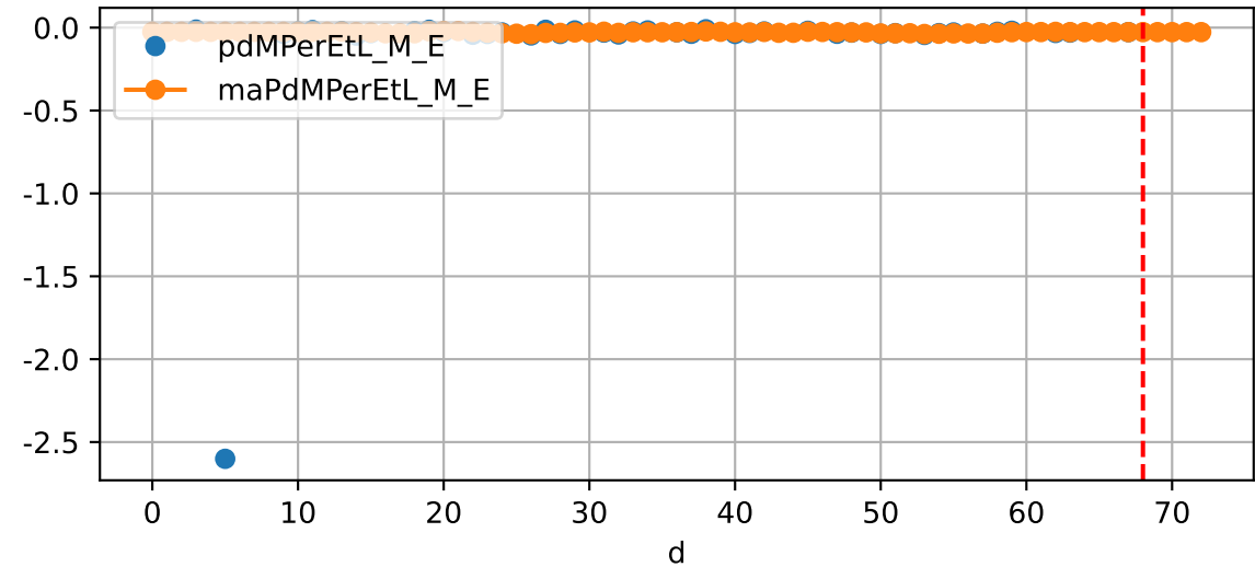
Daily %DeltaM and %DeltaM/1000ml ETcldef for M_E (-4.3%/D, -2.7%/1000ml ET)
