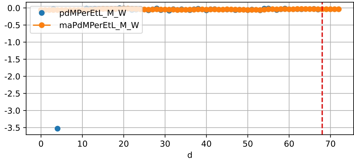
Daily %DeltaM and %DeltaM/1000ml ETcIdef for M_W (-4.0%/D, -3.8%/1000ml ET)
