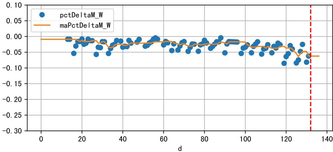
Daily %DeltaM and %DeltaM/1000ml ETcIdef for M_W (-6.2%/D, -6.3%/1000ml ET)
