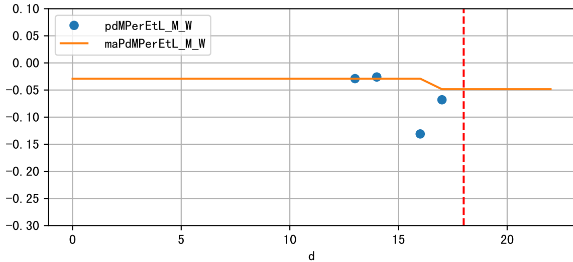
Daily %DeltaM and %DeltaM/1000ml ETcIdef for M_W (-2.0%/D, -4.9%/1000ml ET)
