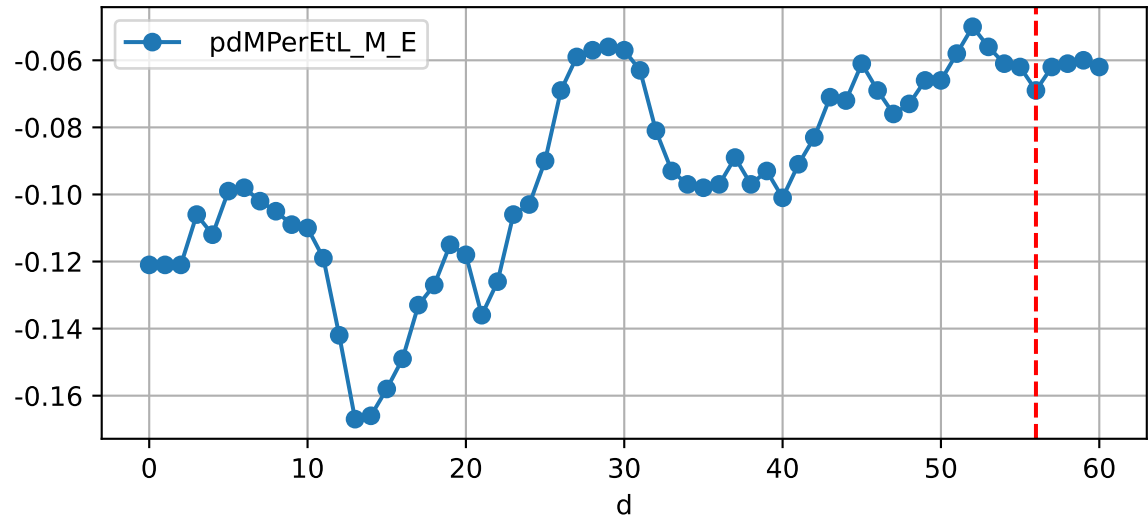
Daily %DeltaM and %DeltaM/1000ml ETcldef for M_E (-9.8%/D, -6.9%/1000ml ET)
