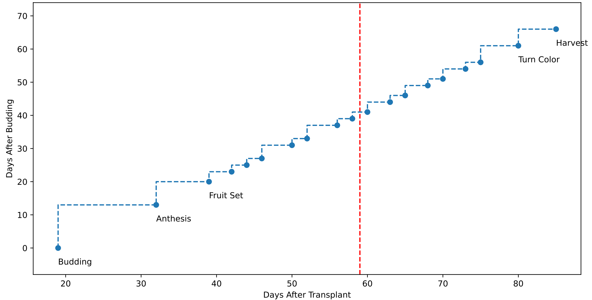
P12 TsN2 (plot by DAT)
