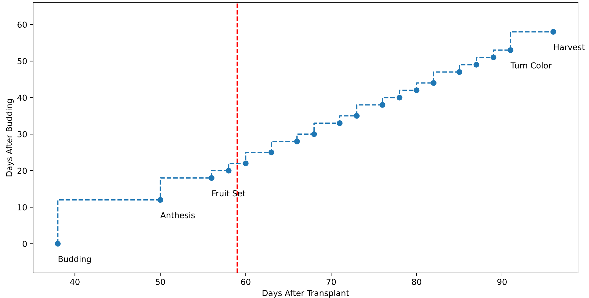
P12 TsN4 (plot by DAT)
