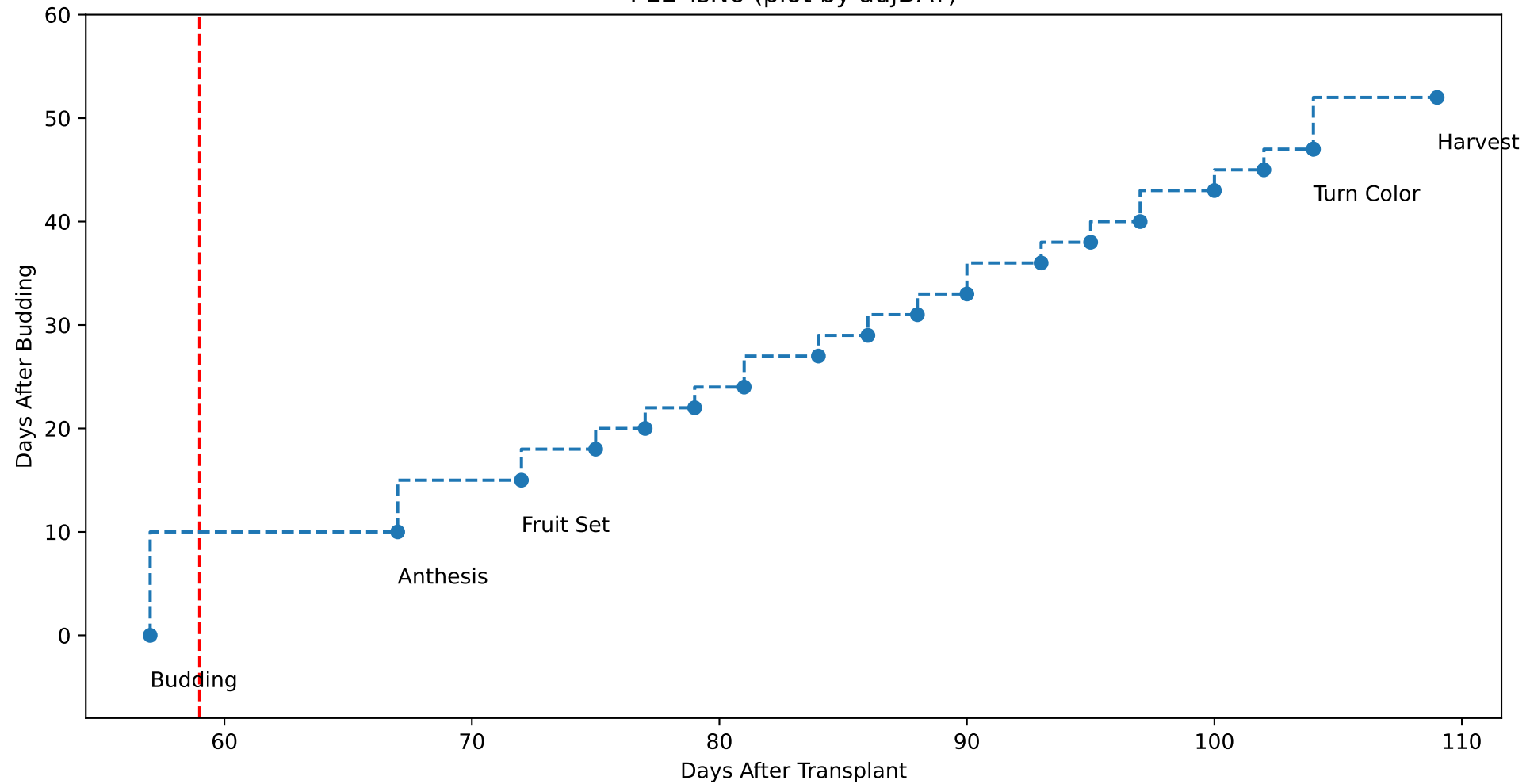
P12 TsN6 (plot by adjDAT)
