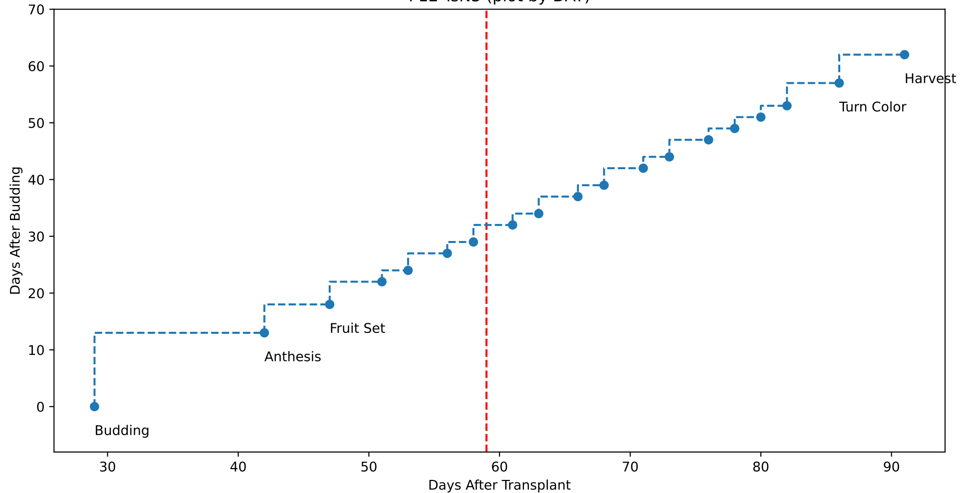
P12 TsN3 (plot by DAT)
