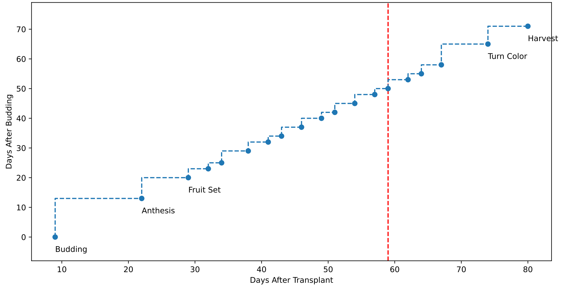
P12 TsN1 (plot by DAT)
