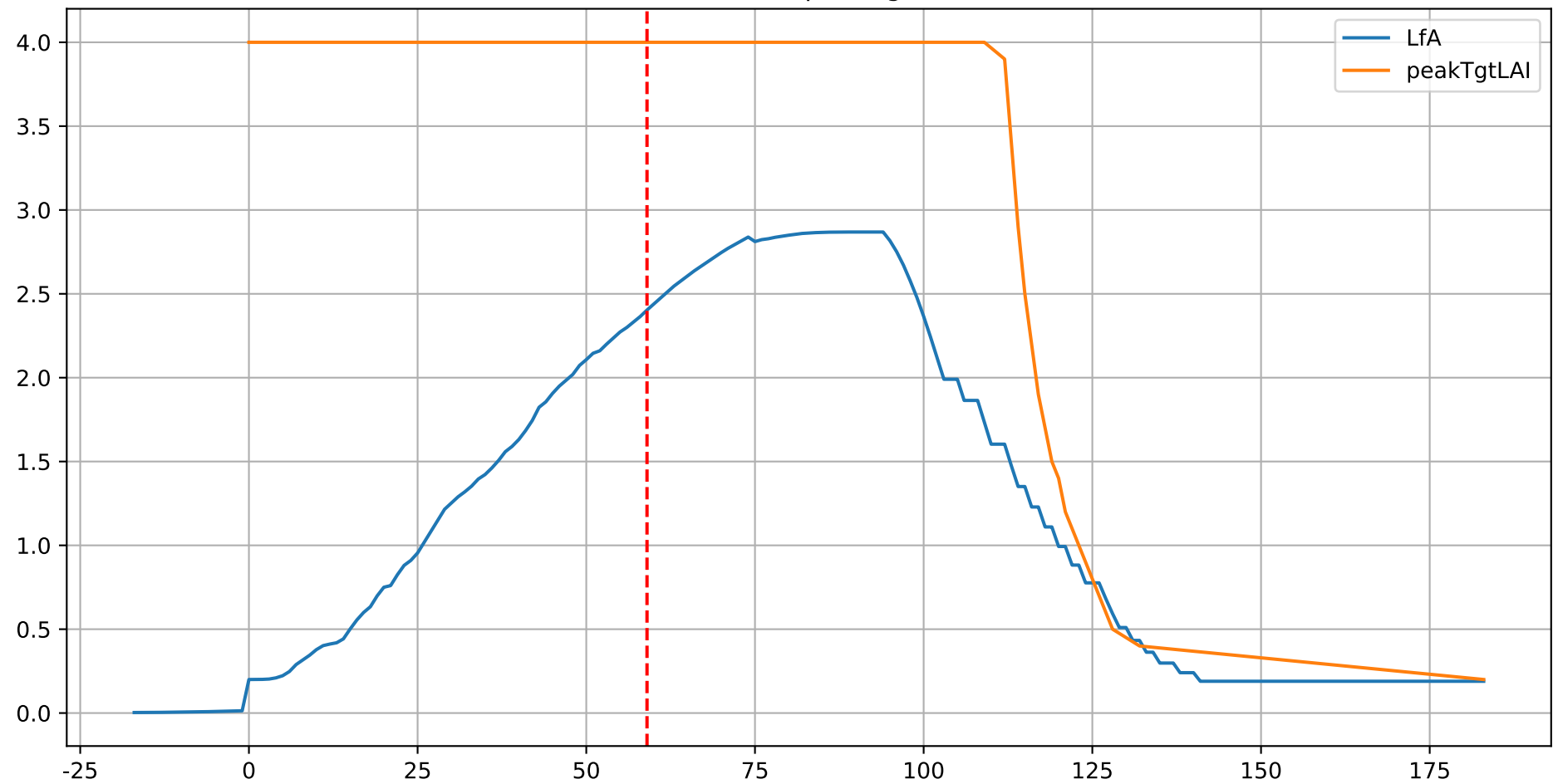
P12: ['LfA', 'peakTgtLAI']
