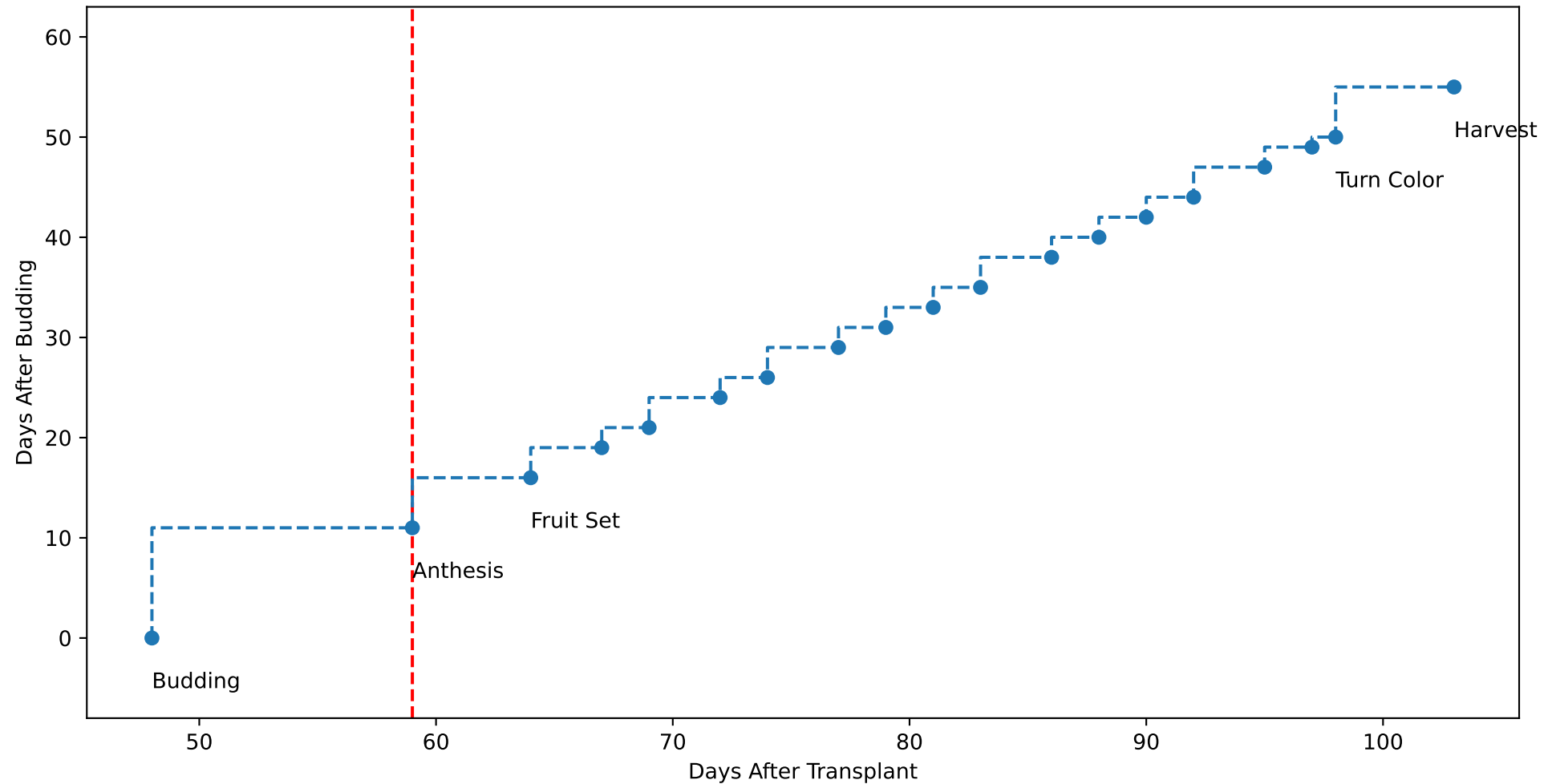
P12 TsN5 (plot by adjDAT)
