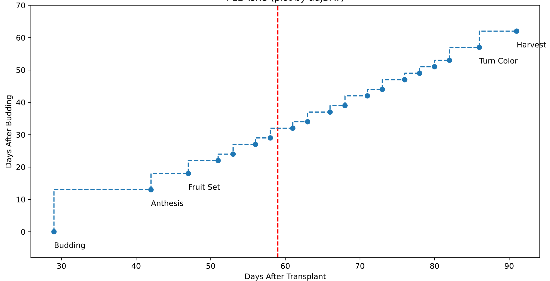
P12 TsN3 (plot by adjDAT)
