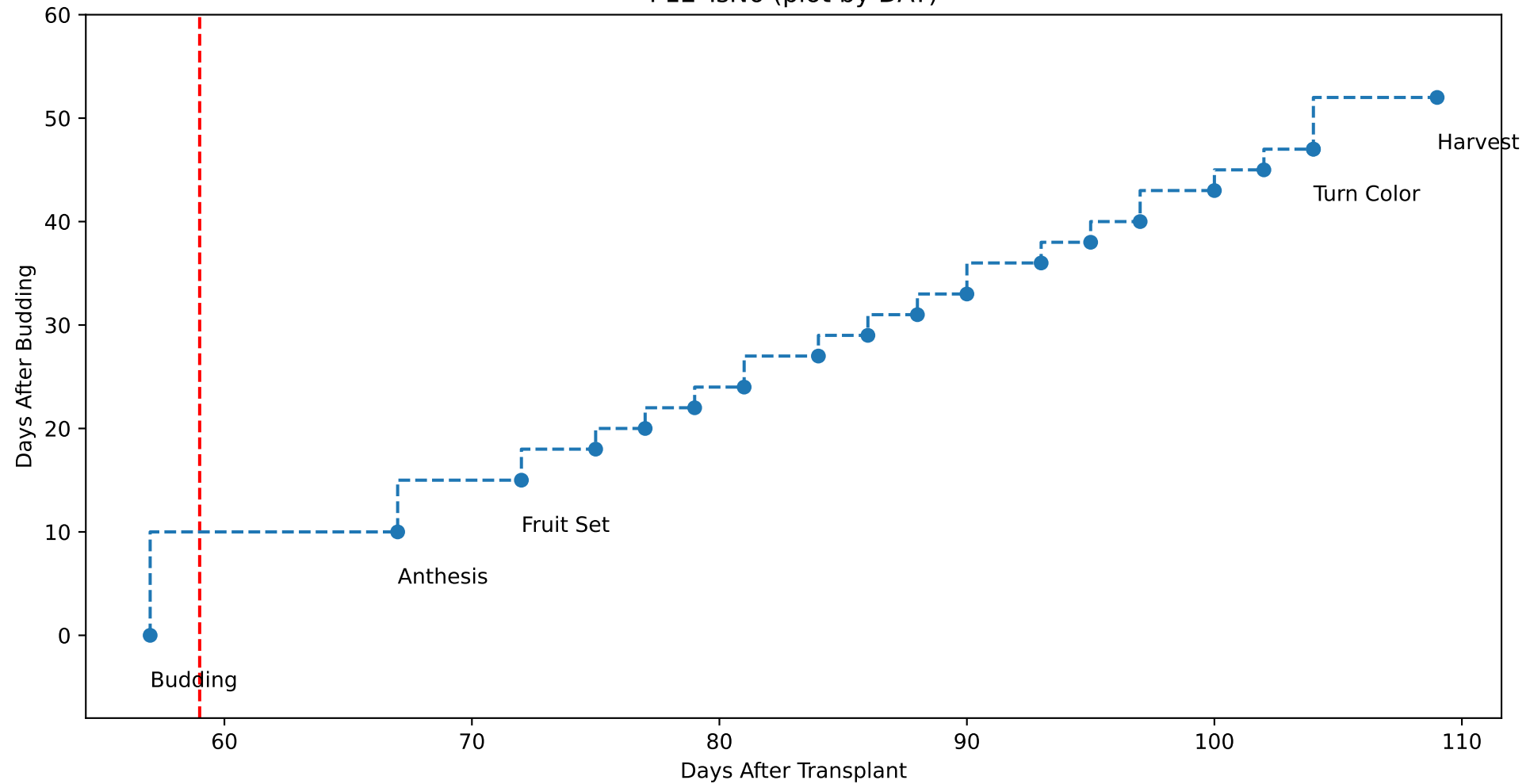
P12 TsN6 (plot by DAT)
