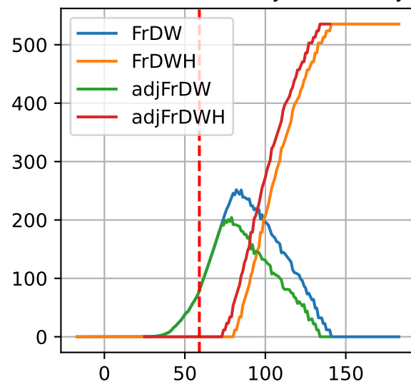
P12: ['FrDW', 'FrDWH', 'adjFrDW', 'adjFrDWH']
