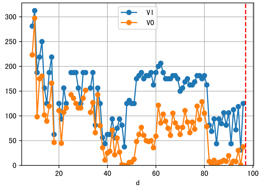
fgNum 2 (at_row = 131)
