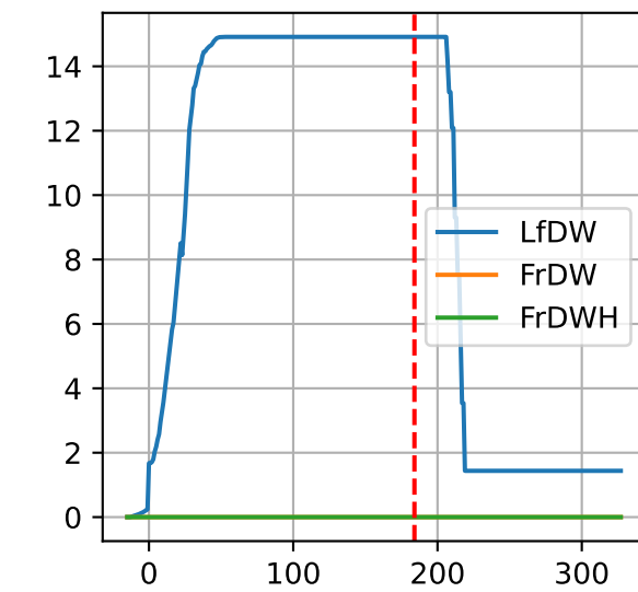
P2-11: ['LfDW', 'FrDW', 'FrDWH'] P2-11: ['FrDW', 'FrDWH', 'adjFrDW', 'adjFrDWH']
