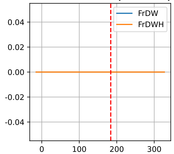
P2-11: ['LfDW', 'FrDW', 'FrDWH'] P2-11: ['FrDW', 'FrDWH', 'adjFrDW', 'adjFrDWH']
