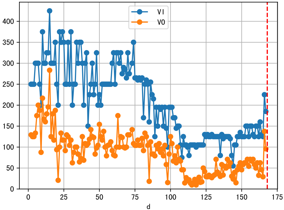
fgNum 1 (at_row = 4)
