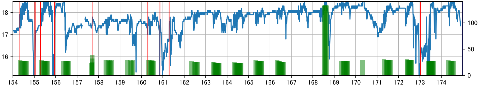
P2A1_0: M_E
