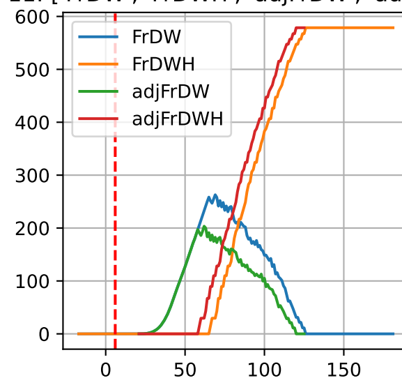
P3-11: ['FrDW', 'FrDWH', 'adjFrDW', 'adjFrDWH']
