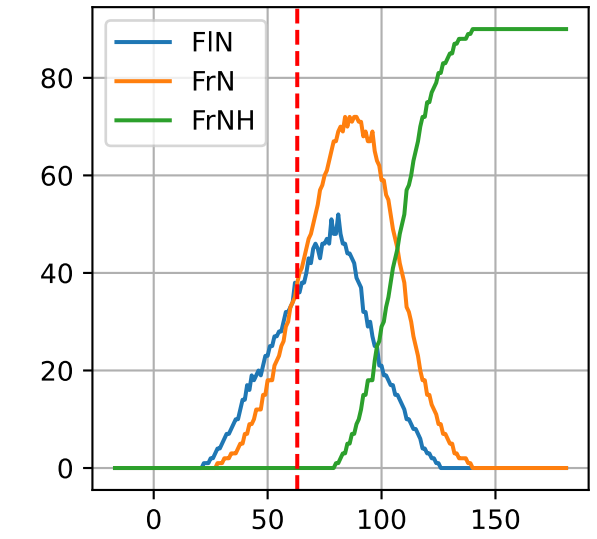
P3-11: ['FIN', 'FrN', 'FrNH']
