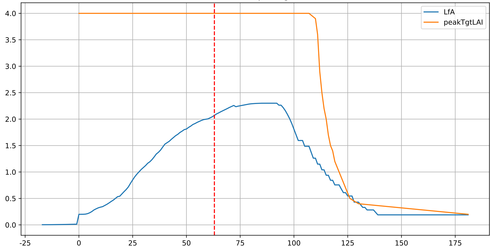
P3-11: ['LfA', 'peakTgtLAI']
