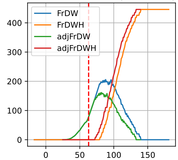
P3-11: ['LfDW', 'FrDW', 'FrDWH'] P3-11: ['FrDW', 'FrDWH', 'adjFrDW', 'adjFrDWH']
