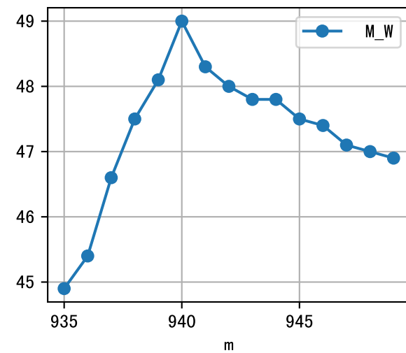
m=935, FV0=0
