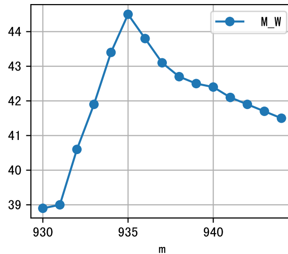
m=930, FV0=0
