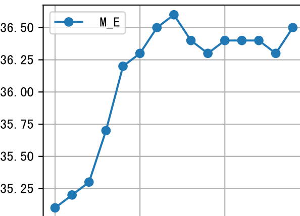
m=740, FV0=0
