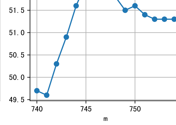
m=740, FV0=0
