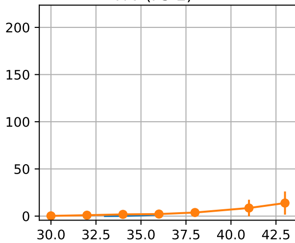
Fit(['S1T1Fr1'], ['S1T2Fr5'])
