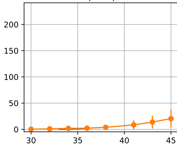
Fit(['S1T1Fr1'], ['S1T2Fr5'])
