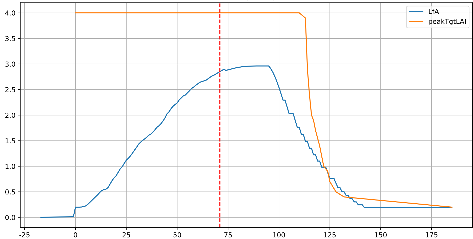
P3-4: ['LfA', 'peakTgtLAI']
