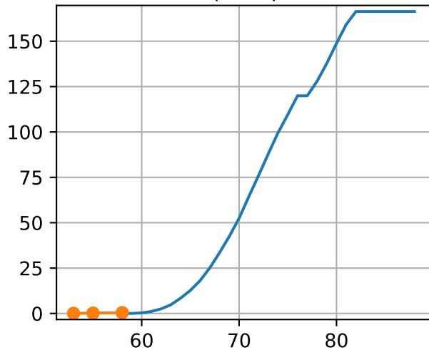
Fit ['S1T4Fr1']
