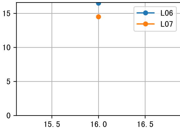
Lfl (P3avg)
