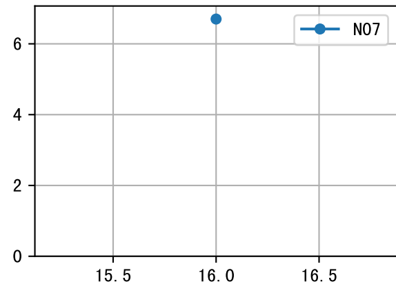
NdD (P3-021-19)
