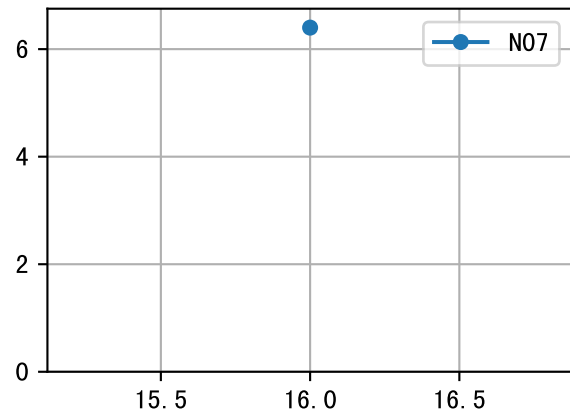
NdD (P3-034-5)
