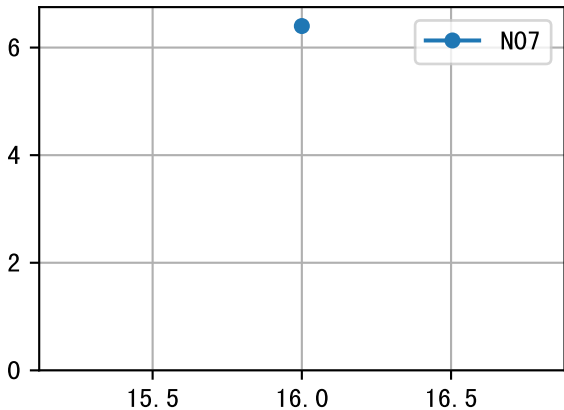
NdD (P3-110-23)
