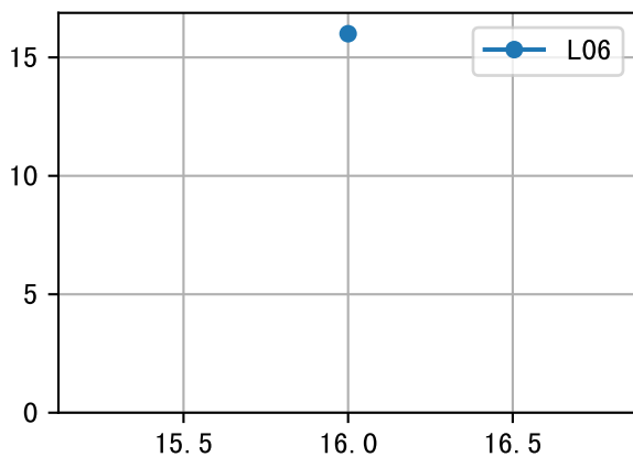
LfL (P3-110-23)
